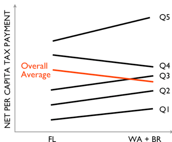
Figure 1: Simpson's paradox
